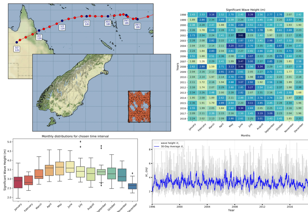
Figure 1: An example of the wave analysis and plotting capabilities of RADWave.
