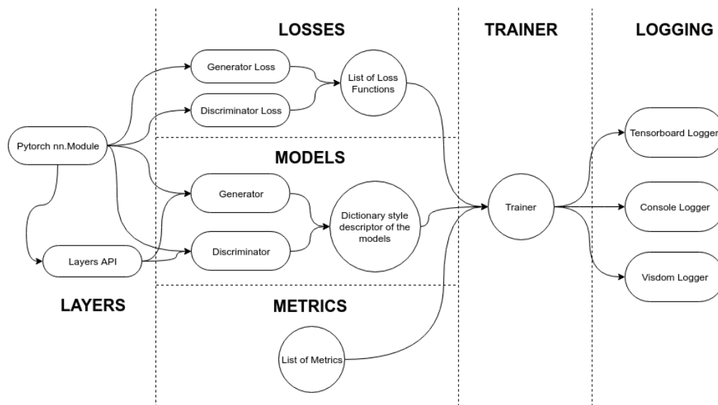
Figure 1: Overview of TorchGAN Design.
