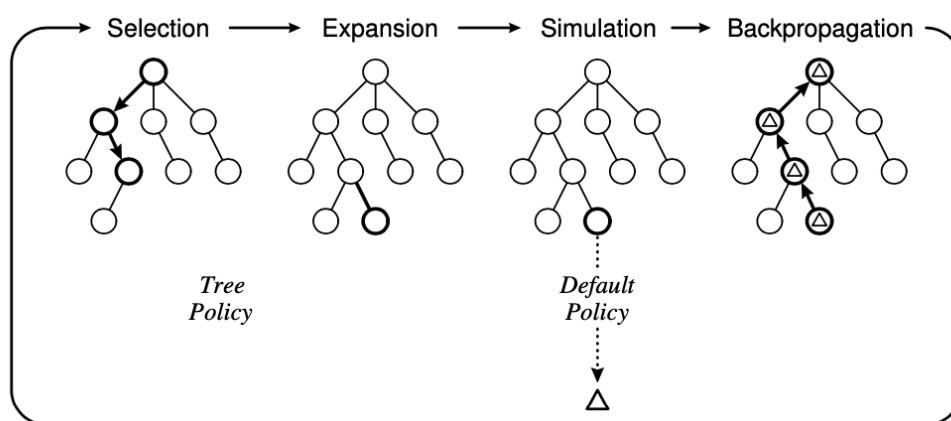
Figure 1: Monte Carlo Tree Search Key Mechanisms. (Browne et al., 2012)
