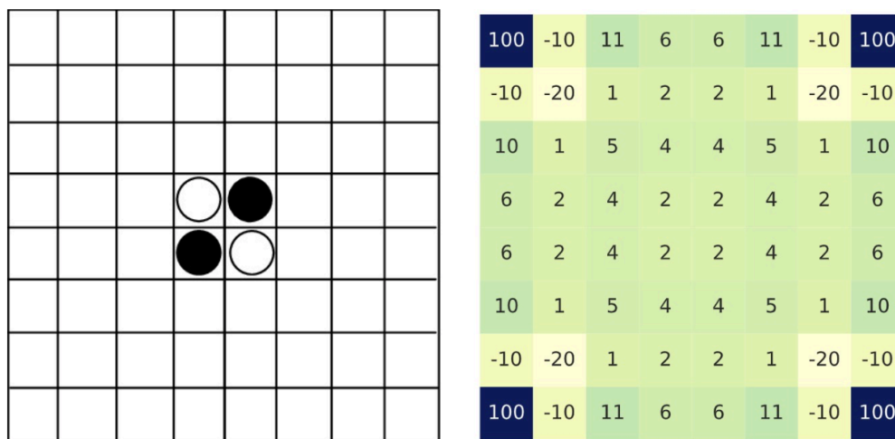
Figure 3: Reversi Heuristic.
