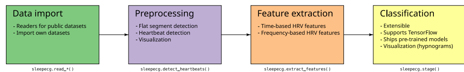
Figure 1: Typical sleep staging workflow.
