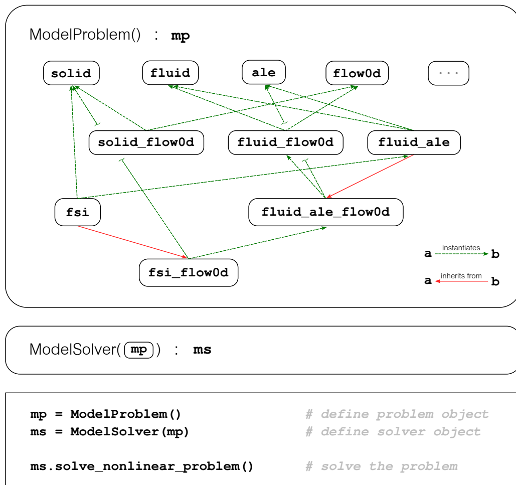
Figure 1: Basic sketch of Ambit code structure: Problem class, solver class, and main code execution flow. Single-physics problems that can be solved encompass solid mechanics (solid), fluid mechanics (fluid), or OD models (flow0d). Two-physics problems like 3D-0D coupling (solid_flow0d, fluid_flow0d), as well as fluid in ALE description (fluid_ale) are defined by instantiating the respective single-physics problems. Three-physics problems arise for coupling of ALE fluid to OD models (fluid_ale_flow0d) or for fluid-solid interaction (fsi), whereas four-physics problems would encompass FSI linked to OD models (fsi_flow0d). Note that the single-physics problem ale just mimics a dummy linear elastic solid and would be irrelevant as a standalone problem.
