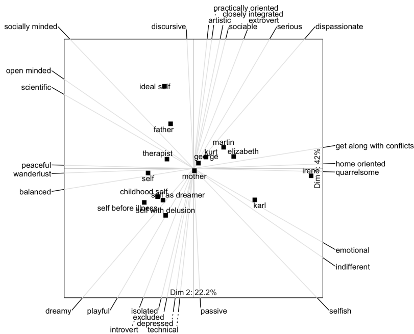
Figure 2: Biplot of Böker's dataset.
