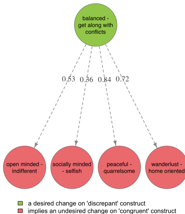
Figure 4: Network graph of implicative dilemmas.
