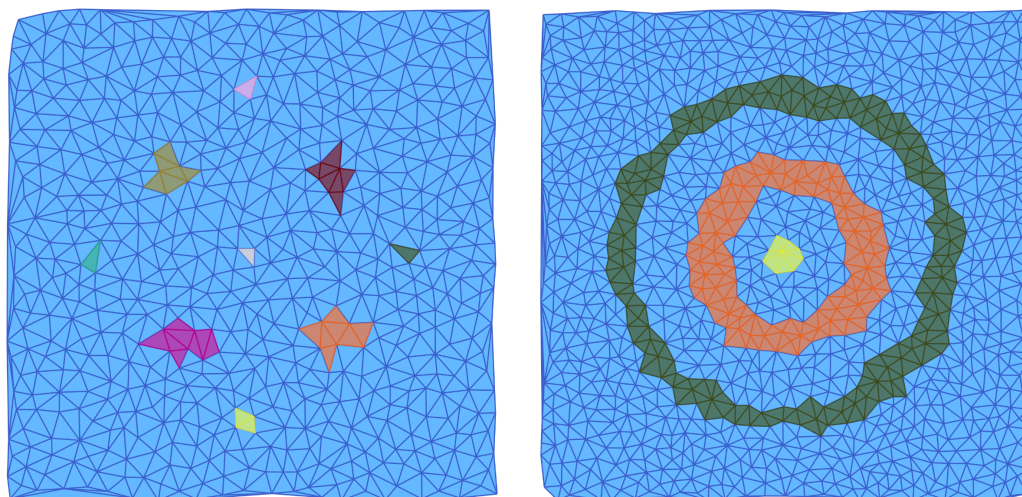
Figure 2: Morse decompositions for the two planar flows shown in the previous figure. In both cases, the underlying Lefschetz complex is a random Delaunay triangulation. The identified Morse sets are shown in different colors.
