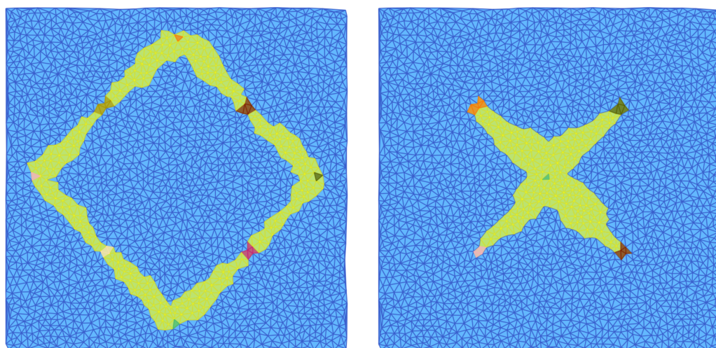
Figure 3: Morse intervals for the planar gradient flow. The yellow regions provide enclosures for heteroclinic orbits in the system.
