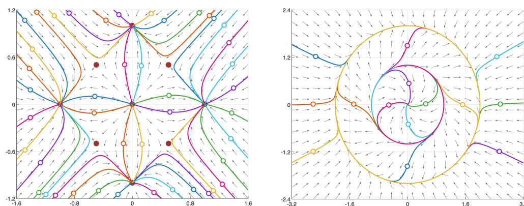
Figure 1: Two sample planar flows. The left image shows a gradient system with nine equilibrium solutions and many connecting orbits between them. The system depicted on the right has one stable equilibrium at the origin and two surrounding periodic orbits.
