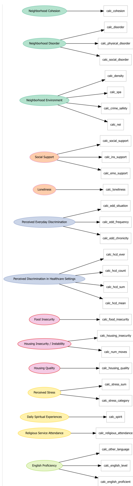
Figure 2: Overview of AOUSDOHtools functions linked to Social Determinant of Health constructs (Koleck et al., 2024). Created with R packages DiagrammeR, DiagrammeRsvg, and rsvg (Iannone, 2016; Iannone & Roy, 2024; Ooms & Bruggemann, 2025).
