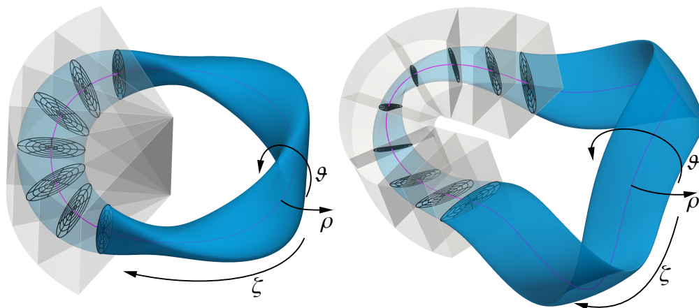
Figure 2: Two examples of stellarator equilibria computed in GVEC, either represented in cylindrical coordinates (left) or in a flexible coordinate frame, following a strongly shaped boundary (right). The flux-aligned coordinates are indicated, with a radial coordinate \rho and two angular coordinates \vartheta and \zeta . In each planar cross-section \zeta = \text{const} , a (\rho, \vartheta) grid (black) is shown, as well as the boundary surface (blue) at \rho = 1 and the magnetic axis (purple) at \rho = 0 .
