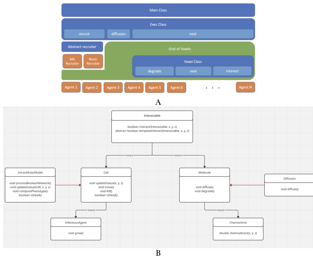
Figure 1: ABM Architecture. A: Overall architecture. The “Exec” iterates through the grid-of-voxels (green) and executes the public methods of Voxel (blue). The Voxels iterates through their local lists of agents (orange bottom), executing their public methods. Exec also executes molecule diffusion, “garbage collection (gc)” of dead cells, and cell recruitment. B: Diagram showing the agent’s classes. Black arrows represent inheritance, while red represents composition. All agents are interactables, which means that they can potentially interact with any other agents.
