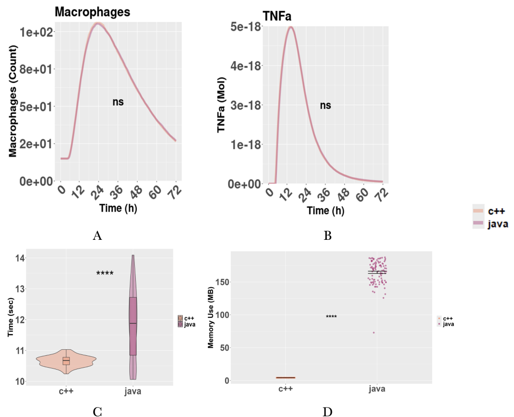
Figure 3: jPAI and PAI++ comparison. A: Macrophage time series. B: TNF-a time series. C: Running time. D: Memory usage. Memory recorded with Valgrind (C++) and JProfiler (Java). All figures represent the average of 100 simulations. Simulations initialized with 10X10X10 voxels, 640 pneumocytes, 1920 conidia, 15 macrophages, and 2160 iterations. PAI++ compiled with g++ 12.4.0 using the MinGW toolchain with level three optimization; jPAI run with Java 23.0.1. Execution environment: Windows 10 Education 64-Bit Dell laptop, Intel® Core™ Ultra 7 155U (14CPUs), ~2.1GHz, 16384MB RAM. A-B: paired t-test. C-D: Wilcoxon rank-sum test. (ns not significant p > 0.05 ; **** p < 0.0001 ).
